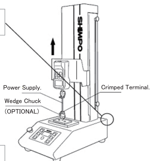
(Example) Tension Test of Wire.
