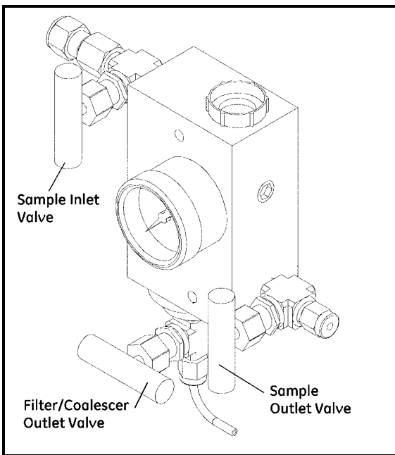
Figure 13: Sample System Valve Locations
