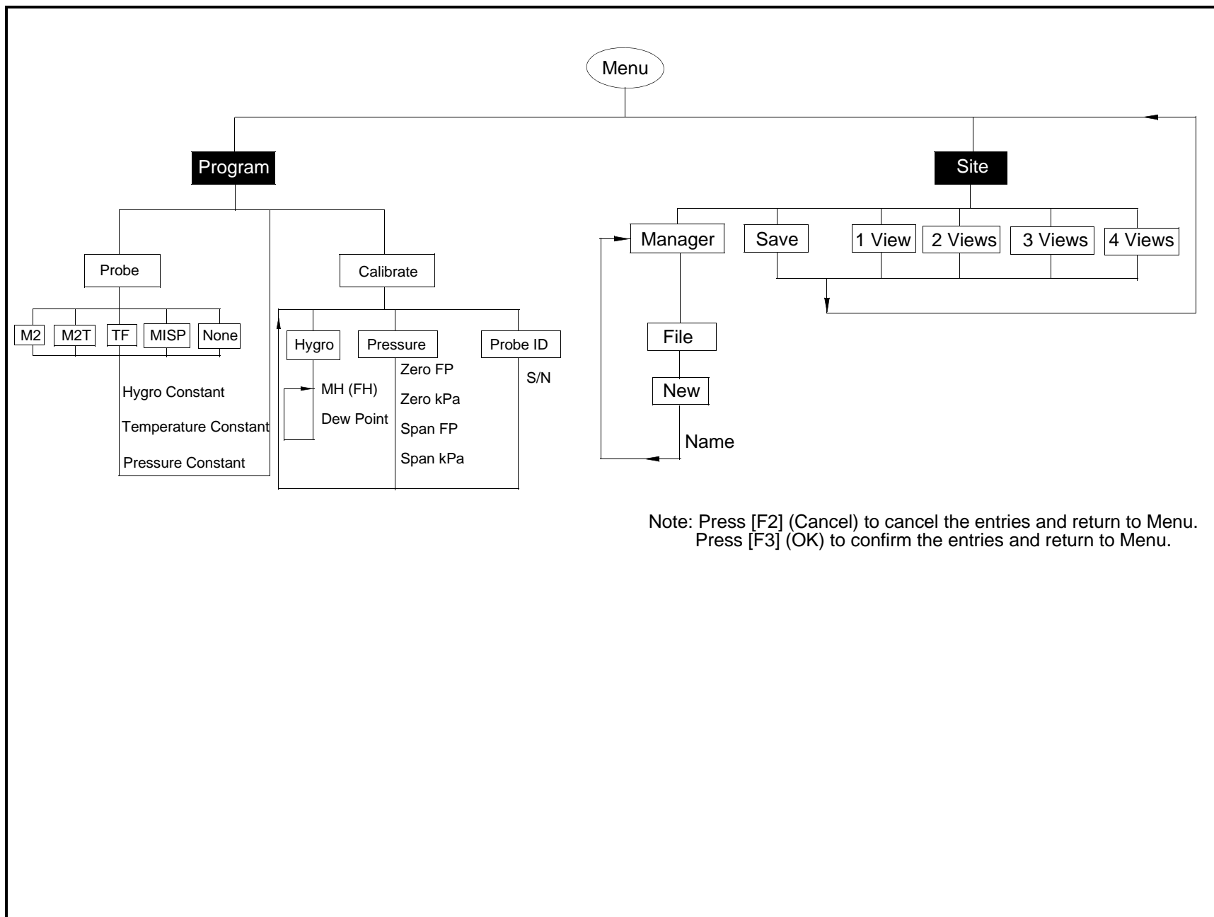
Figure 9: Startup Menu
