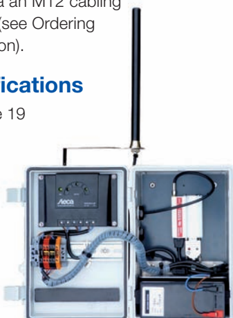
GP2-BX1/SP modem box (solar panel not shown)
